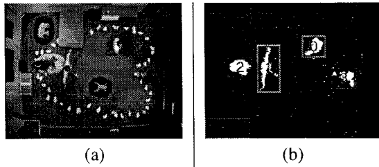
Figure 1. (a) The top-down view of the KidsRoom used by the real-time tracking algorithm. Four people and a movable bed are in the room. (b) By using a fast, simple clustering algorithm, small background difference clusters are merged with larger nearby clusters, as marked by the bounding boxes.
